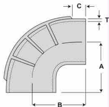
90° Elbow
