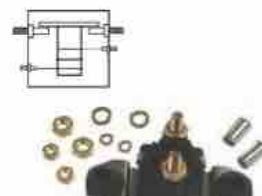
18-5820 SOLENOID
