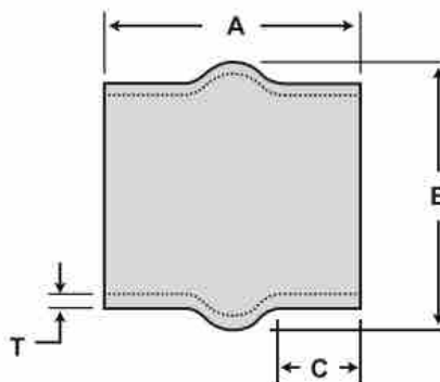
Hump Hose
