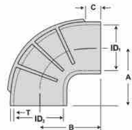
90° Reducing Elbow
