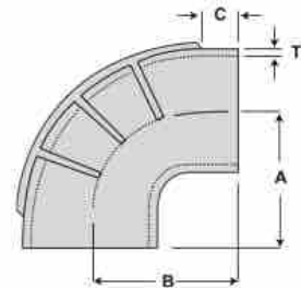
90° Elbow
