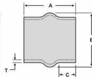
Hump Hose
