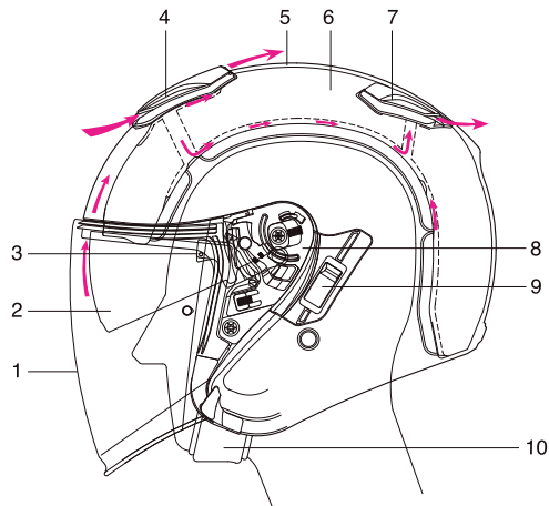
Anti-Condensation Shield Ventilation System
