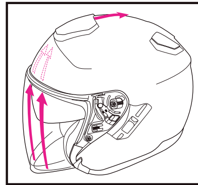
Anti-Condensation Shield Ventilation System
