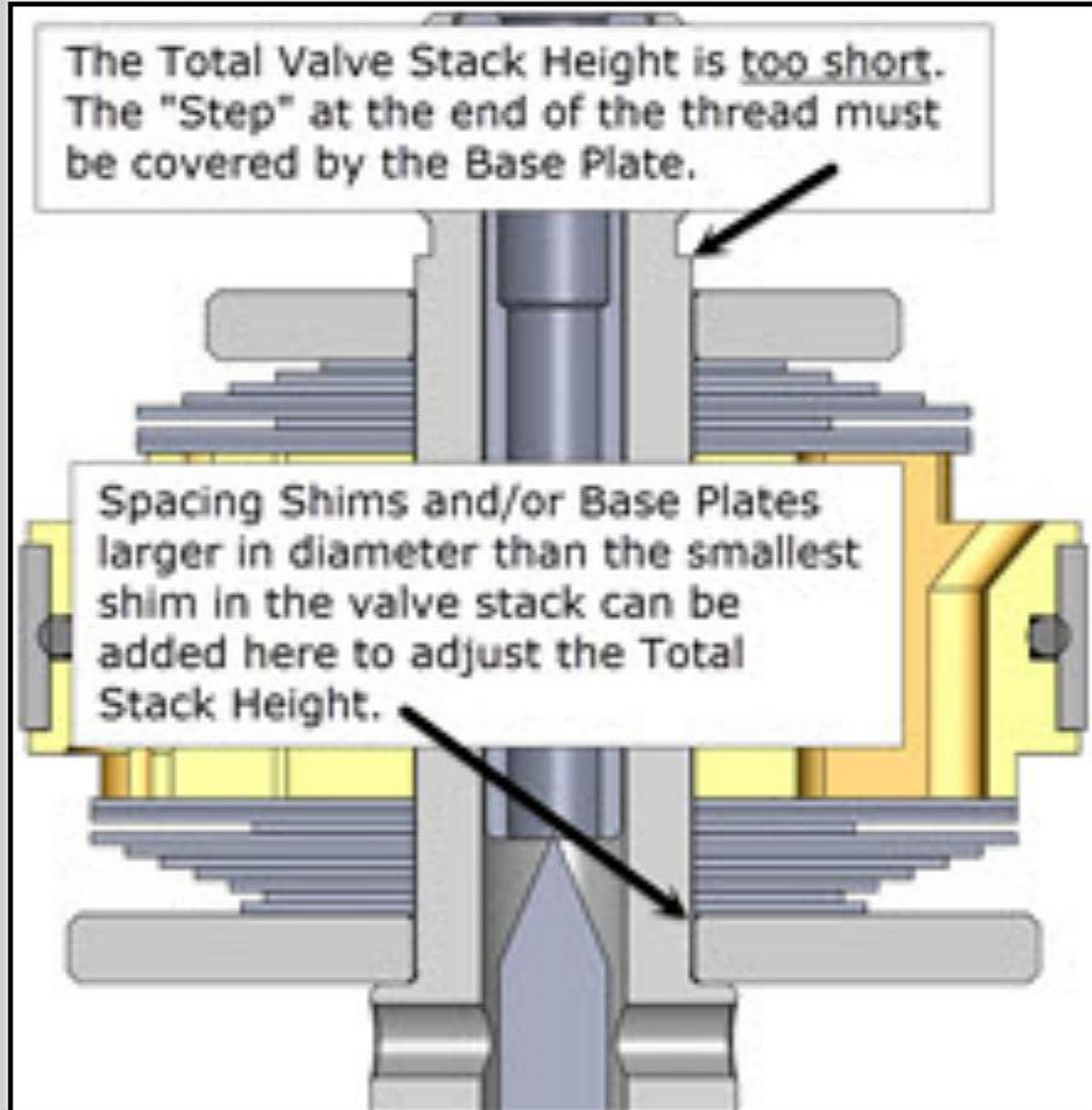
Incorrect stack height is shown in this photo (this stack is too short).
