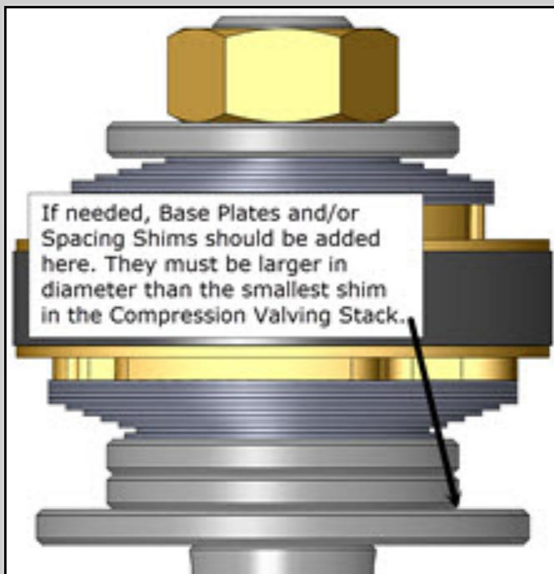
Base Plates can be added if required.
