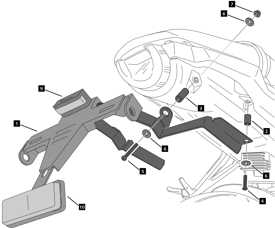
Fixation license support rotation (2 OPTIONS A-B)
