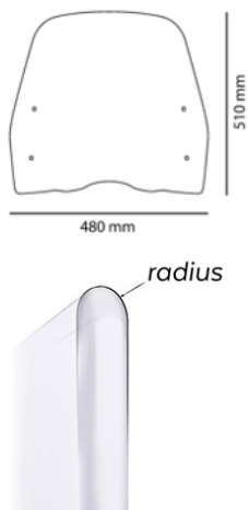
ROUNDED CONTOUR-PROFILE
