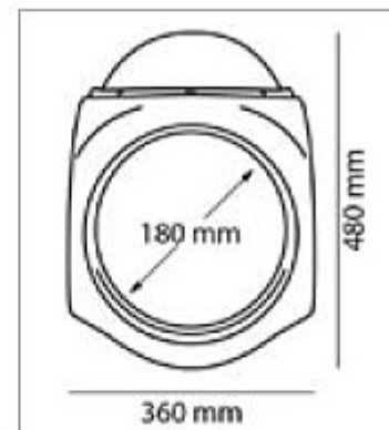
2 fixing points
