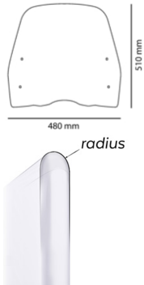
ROUNDED CONTOUR-PROFILE
