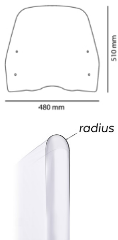
ROUNDED CONTOUR-PROFILE
