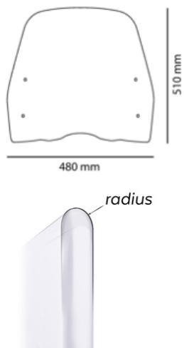
ROUNDED CONTOUR-PROFILE
