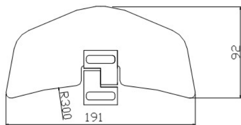
DEFLECTOR 2
