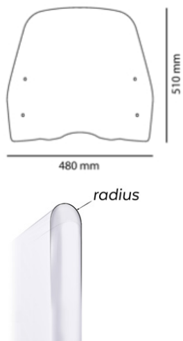
ROUNDED CONTOUR-PROFILE
