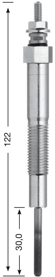
Y-529 J M 10 x 1.25 12 Hex 11 V
