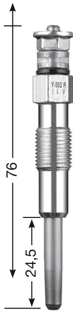
Y-502 R M 10 x 1.0 10 Hex 11 V
