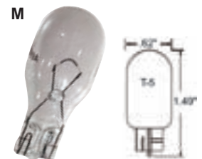
Wedge Base
