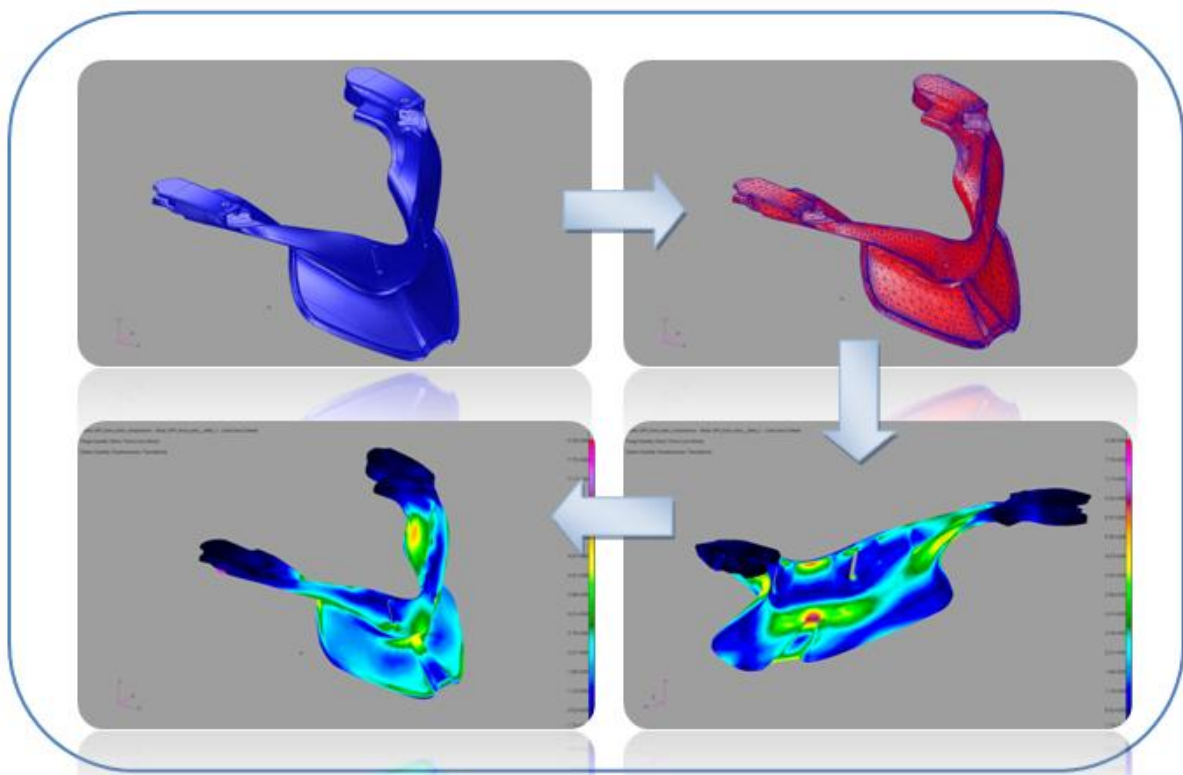
Figure 4-44: FEM of the lower front of the device
