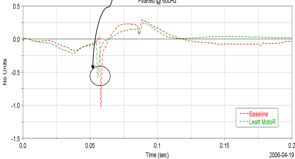
Figure 4-10: Nij obtained through testing and simulation
