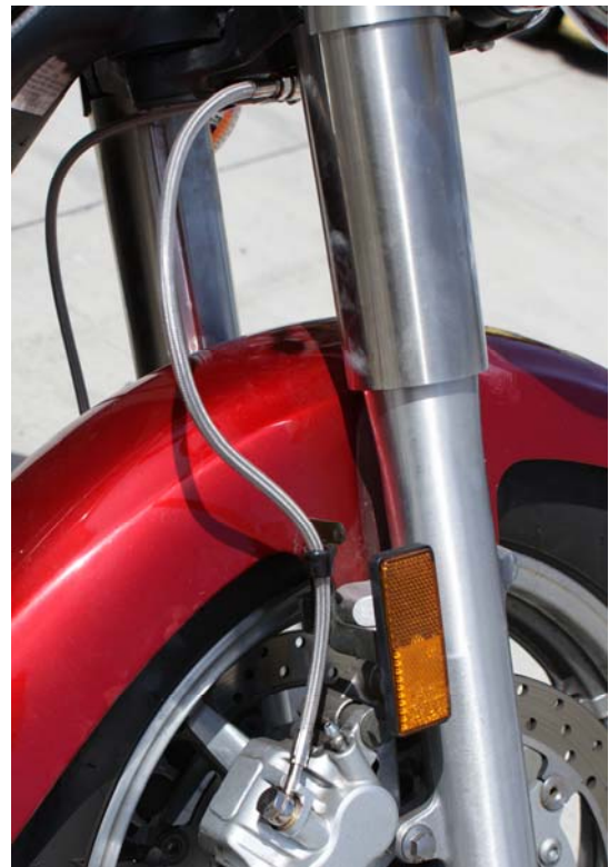
d. Line B – Right caliper routing
