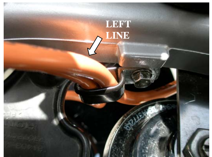
d. Galfer provided c-clip at lower triple tree
