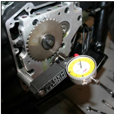
Engines that have extreme cam chain pad wear, inspect crank sprocket for side to side runout. The registry may need to be modified to help extend pad wear
