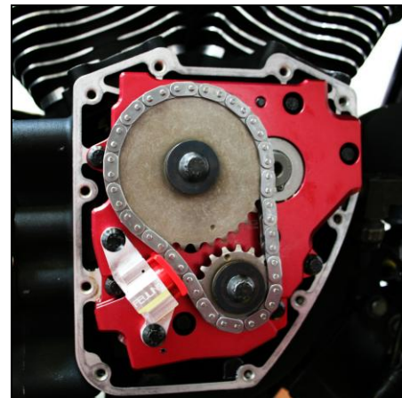
Feuling outer cam chain, tensioner, sprockets cam/crank bolts and washers installed
