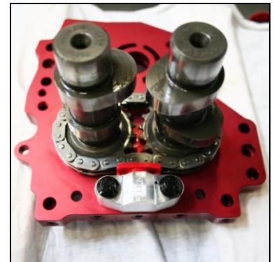
Inner cam chain + tensioners installed into '07-'16 camplate
