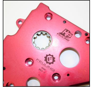
Set camplate into proper fixture to press roller bearing into camplate, verify bearing is pressed square and flush with camplate
