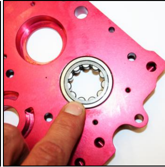
Set camplate into proper fixture to press roller bearing into camplate, verify bearing is pressed square and flush with camplate
