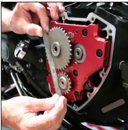
Align sprockets using a straight edge to verify correct spacer behind rear cam sprocket. Note: Front cam uses 0.100" thick thrust washer
