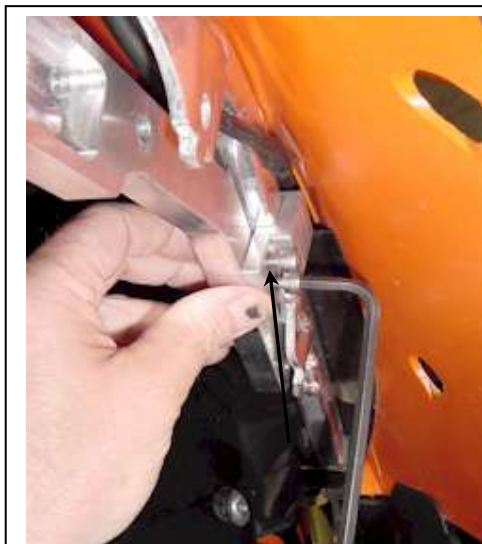
Figure 11: RH sub frame bracket clamp
