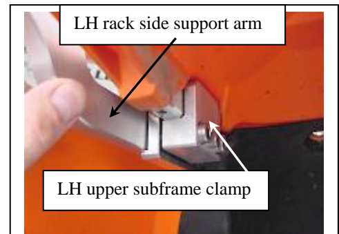
Figure 13: LH upper clamp and side arm install
