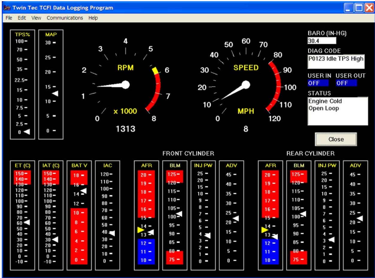
Figure 18 – Real Time Engine Data Display
