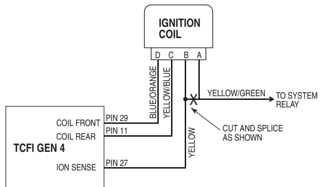
Figure 25 - Sportster® Ion-Sense Wiring Modification at Ignition Coil
