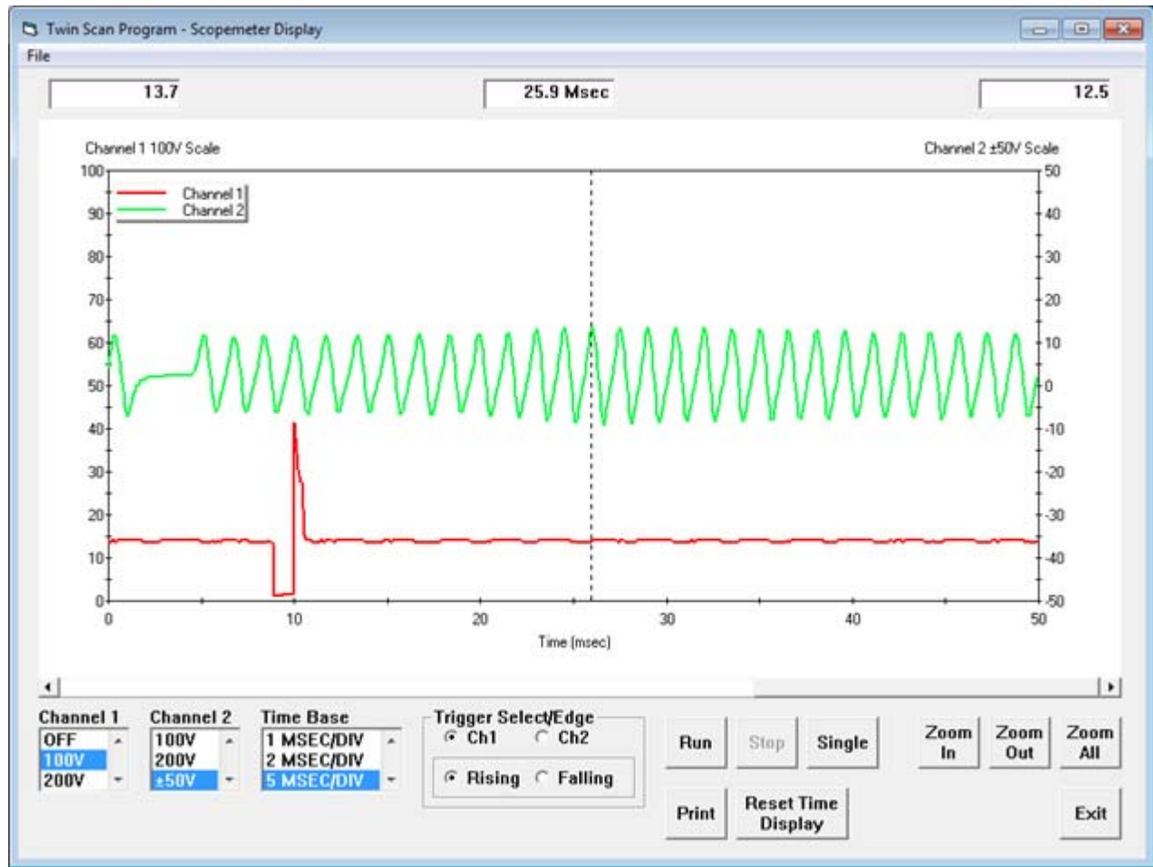
Figure 18 – Scopemeter Display
