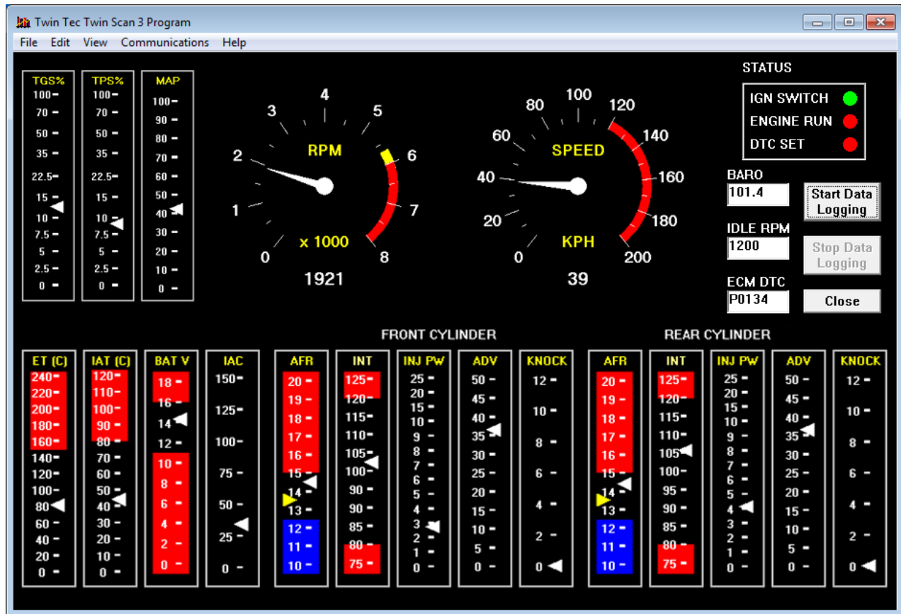
Figure 8 – Real Time Engine Data Display
