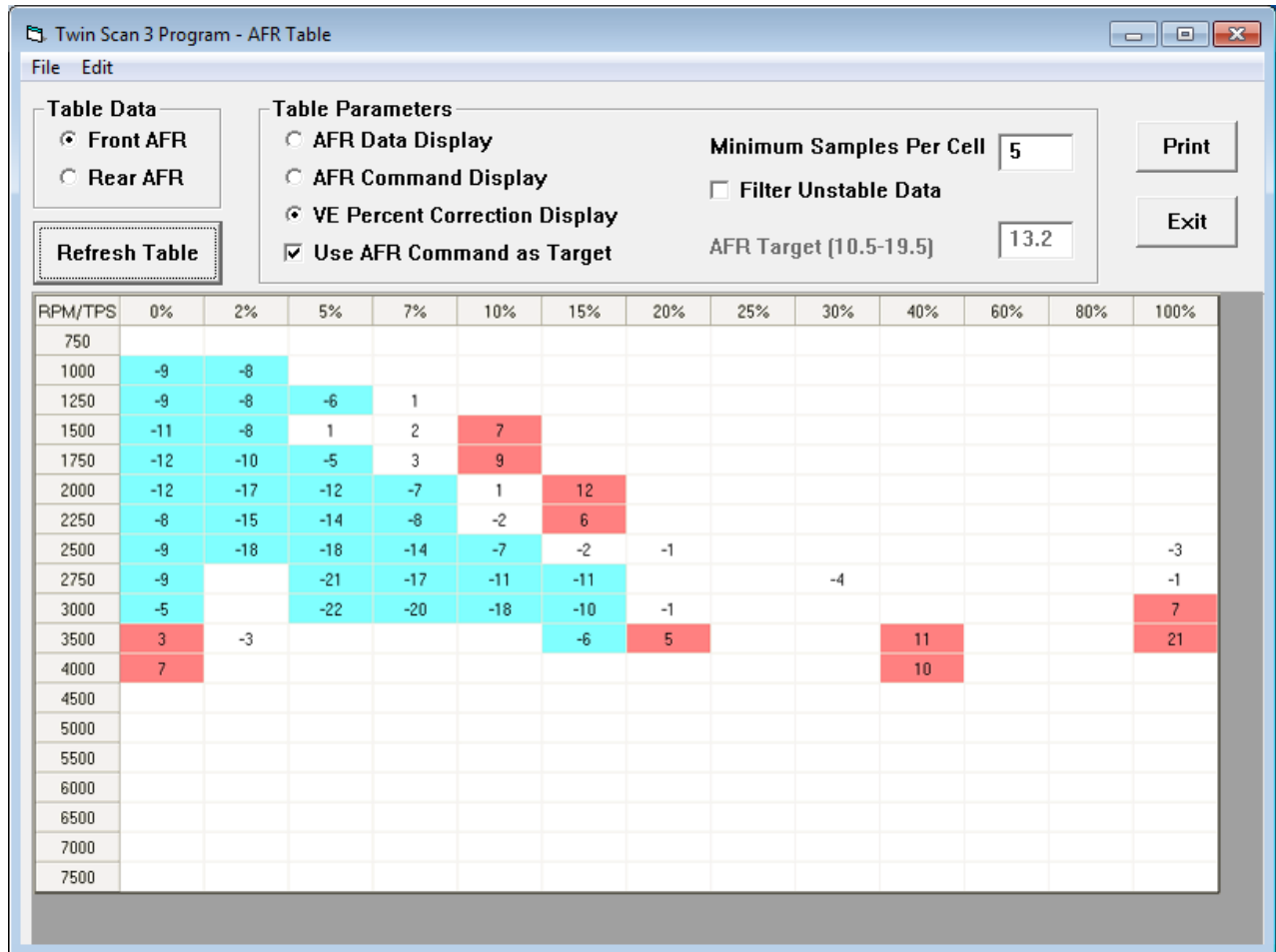
Figure 13 – VE Percent Correction Display
