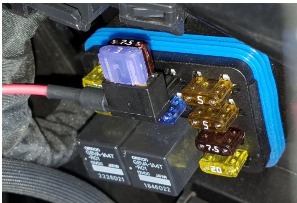
Figure 16B – SYSTEM 7.5A Fuse tap connection for switched uninterrupted power
