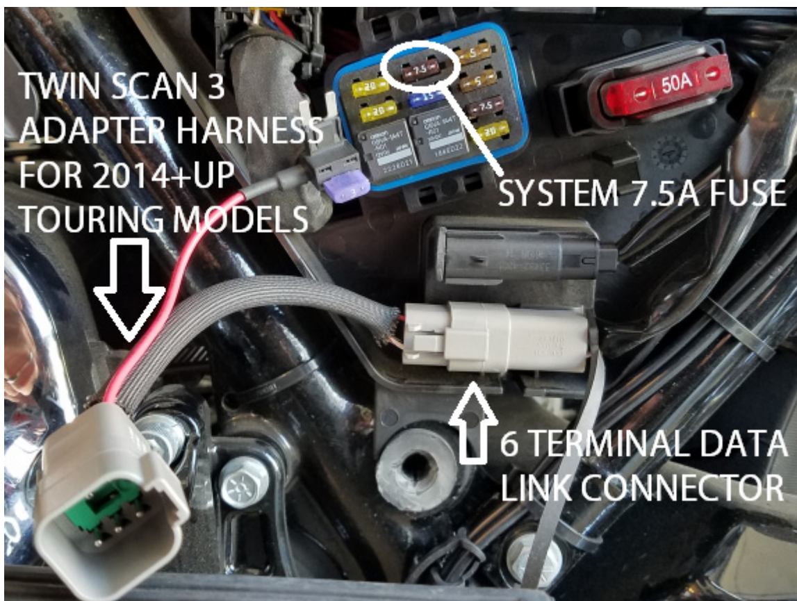
Figure 16A – Adapter Harness connection for 2014-up Touring Models
