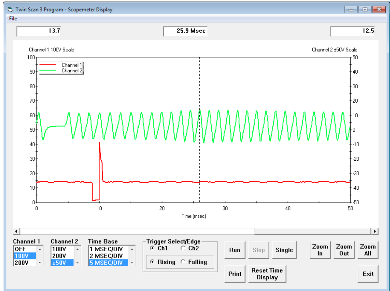
Figure 15 – Scopemeter Display
