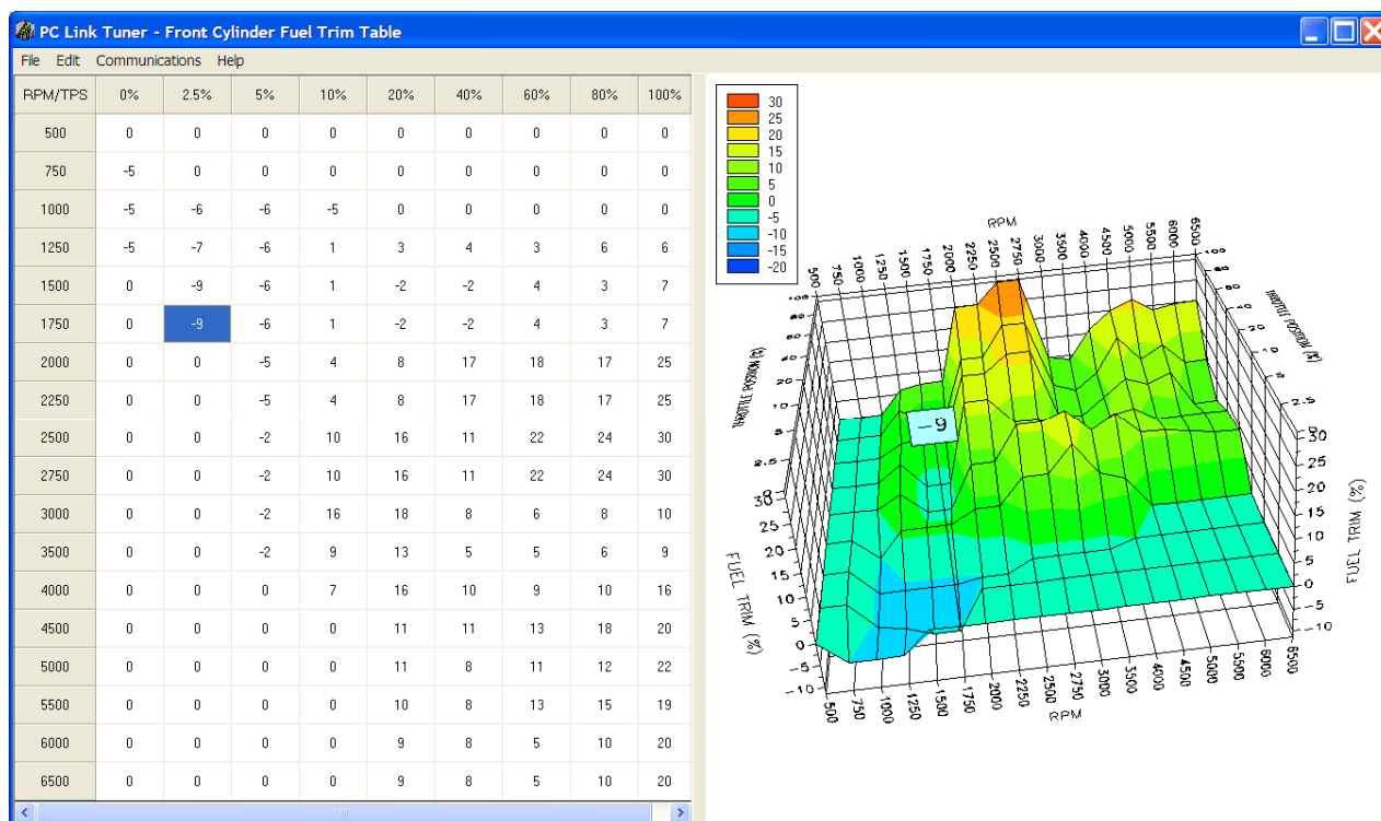
Figure 14 – Twin Tuner Fuel Trim Table
