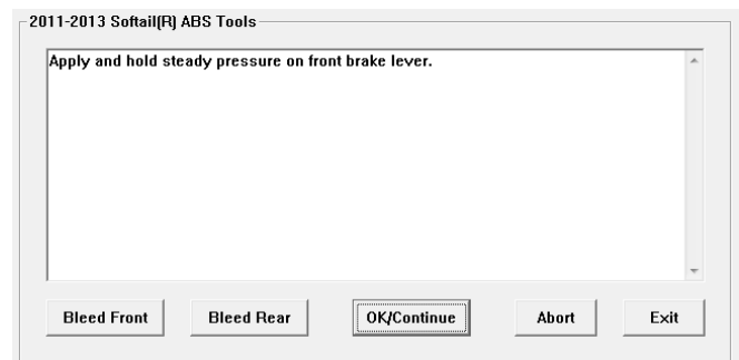
Figure 5 – ABS Tools
