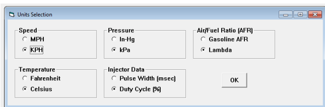
Figure 7 – Units Selection
