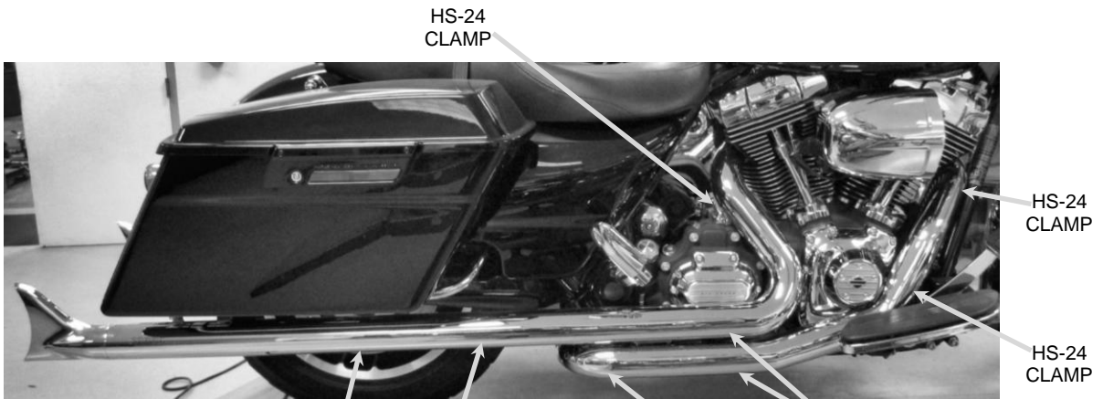
HS-28 CLAMP HS-24 CLAMP FIGURE 7 HS-24 CLAMP HS-24 CLAMP
