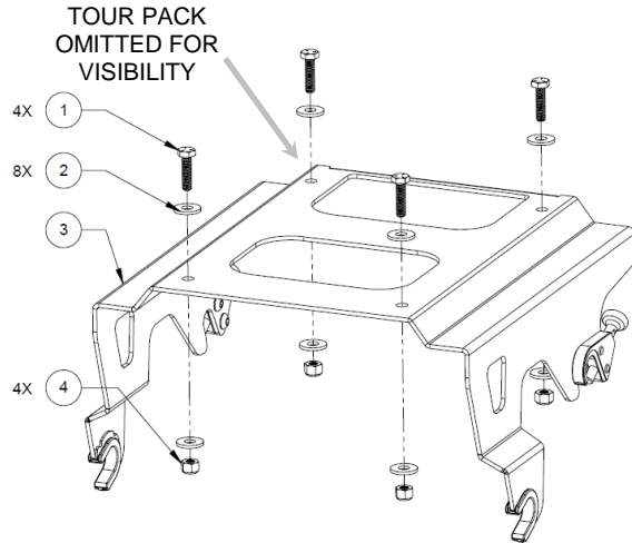
FIGURE 2, HARDWARE INSTALLATION
