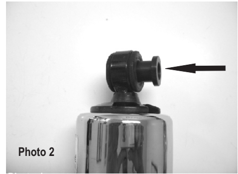
Photo 2 Instal a shouldered sleeve as shown into each mounting eye of both shocks
