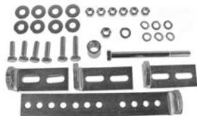
GDR9104 Universal Mounting Kit Includes (4) Cast Steel Brackets, (1) Bolt Spacer, and Hardware Used to Mount Alternators in Place of Generators
