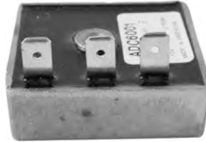
ADC6001 Voltage Regulator For Ducati M/Cs 15mm H x 42mm W x 44mm L Used on Aprilia, Benelli, Betamoto, Ducati, Laverda, Malaguti, Rieju, Others REPL.: APRILIA AP8212119, -121; DUCATI 343301, 34330116
