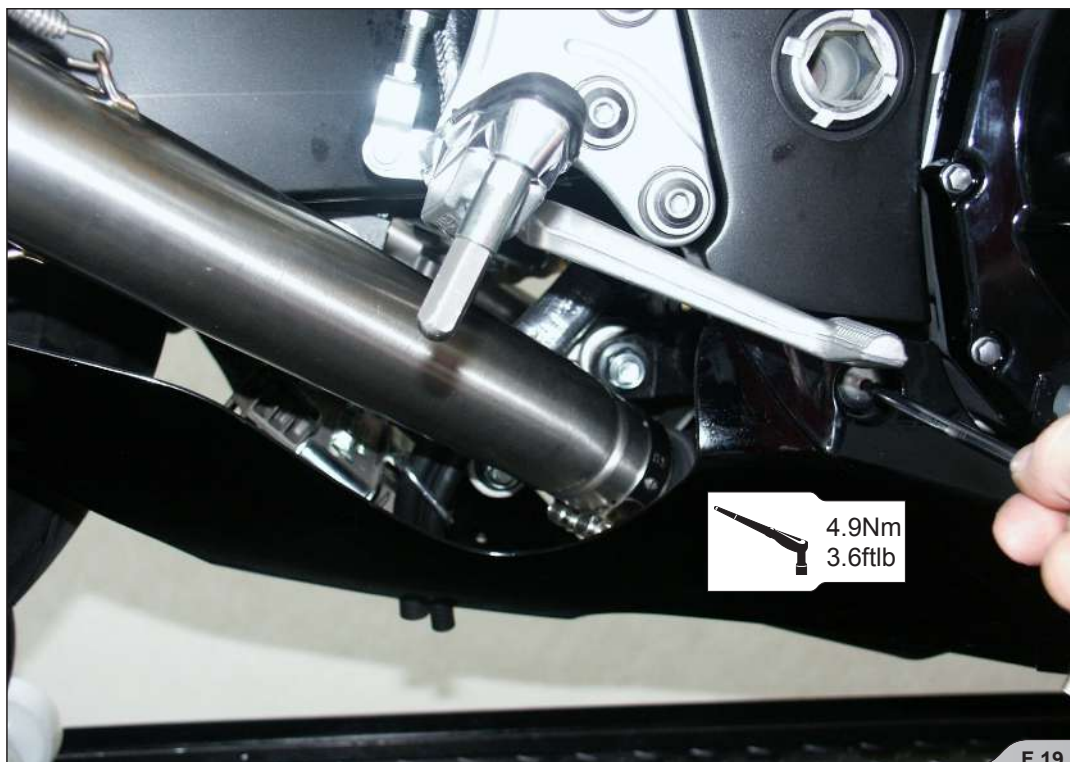
10. Position of the correctly installed Akrapovic SLIP-ON system (F 20).
