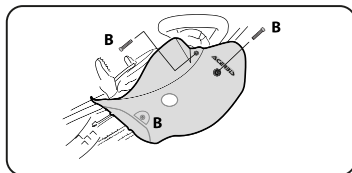
6. Introduce the screw B in the bracket F with out tighten it, then the lateral screw B, and finally tighten all screws B.
