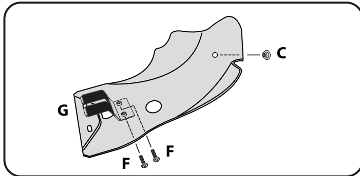
3. Mount the bracket G on the skid plate using the screws F. Introduce the bushing C.
