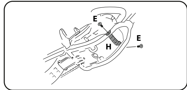
4. Mount the bracket H on the frame using the screws E.
