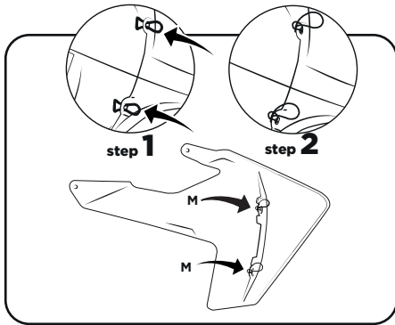
7. Fasten the O-rings M to the radiator scoops, as shown.
