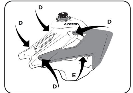
9. Remounting the radiator scoops with 4 screws D and 2 screws E.
