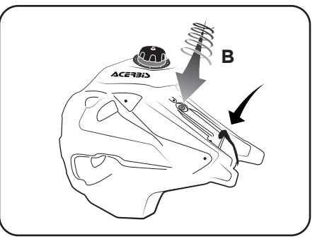
5. Arrange the tank on the bike, reconnect the fuel pump power cable and screw the tank screw B back on.
