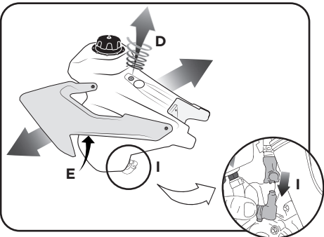
2. Remove the radiator scoops, the seat screw and the Husqvarna tank.
