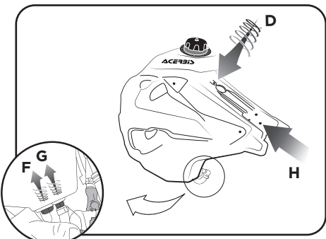
4. Insert the seat screw D (2,5KN - 22INH), fasteners F/G on the Acerbis fuel tank and reconnect the fuel connector by screwing the four pump screw H (3KN - 26INH).
