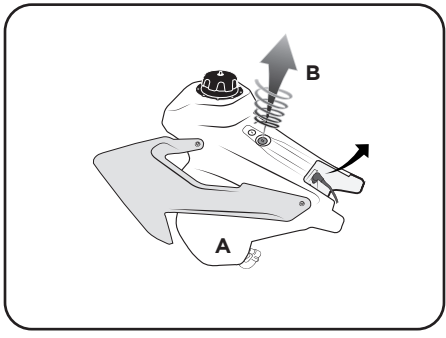
1. Remove the tank screws B. Disconnect the fuel pump power cable.
