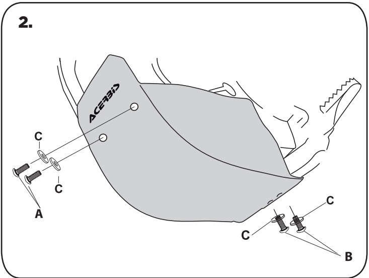
2. Put the skid plate and screw the screws.
