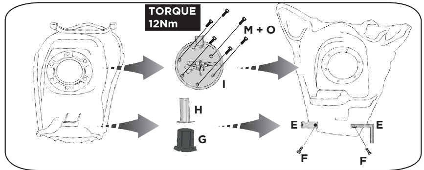
4. Remove the original tank rubber G+H, the pump and reassemble using closing torque 12 Nm, fixing the pump with the screws M and washers O. Fix on the tank the brackets E by the screws F.
