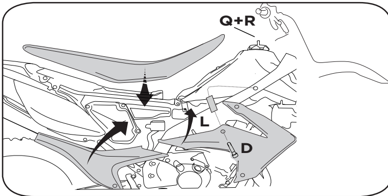
11. Mount plastics and the seat. Use the screws D and the bush L for fix the central hole of the radiator scoops. Fix the Q Pipe on the cup and on handlebar by the R plastic bracket .
