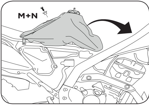
7. Fix the seat bush N by the screw M and Mount Acerbis tank on the bike.
