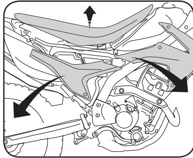
1. Remove the seat and plastics
