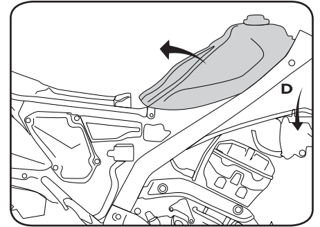
2. Remove the original tank: two screws D that fix the tank, will be used for fix the radiator scoops.
