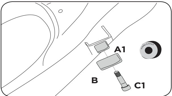
5. Mount all the brackets Rh on the frame (the B rubber must be fix with the "ACERBIS PLASTICA" outside)
