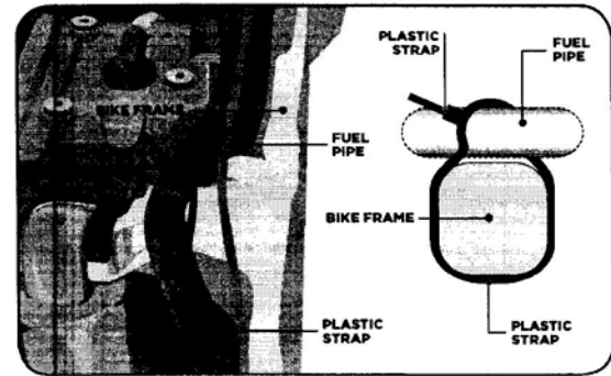
6. Fix the fuel pipe on the bike frame with the plastic strap.
