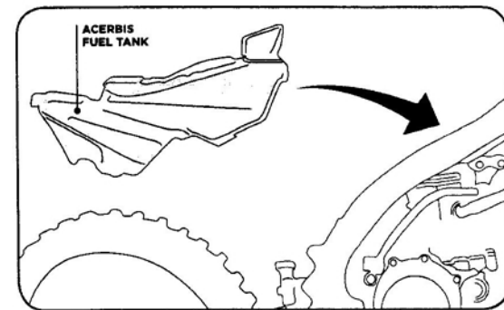
8. Mount acerbis tank
