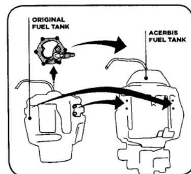
7A. Disassemble and reassemble the pump on the acerbis tank
