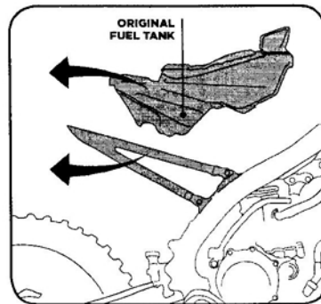
5. Remove the original tank and rear subframe
